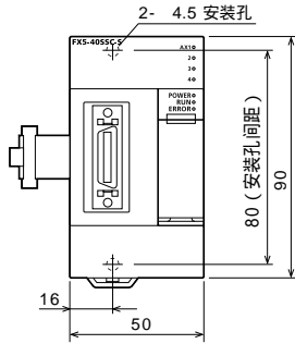
FX5-40SSC-S / FX5-80SSC-S
