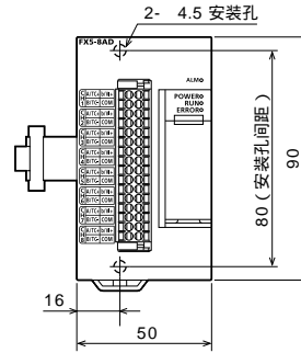
FX5-8AD
