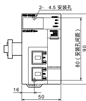
FX5-CCLIEF
