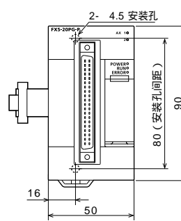
FX5-20PG-P
