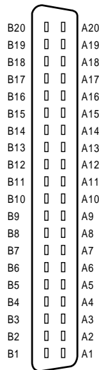
FX5-20PG-P
