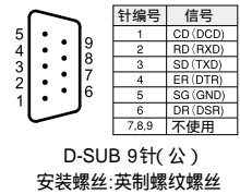
FX5-232ADP
