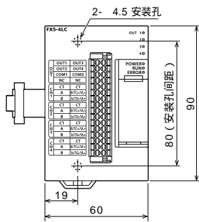
FX5-4LC
